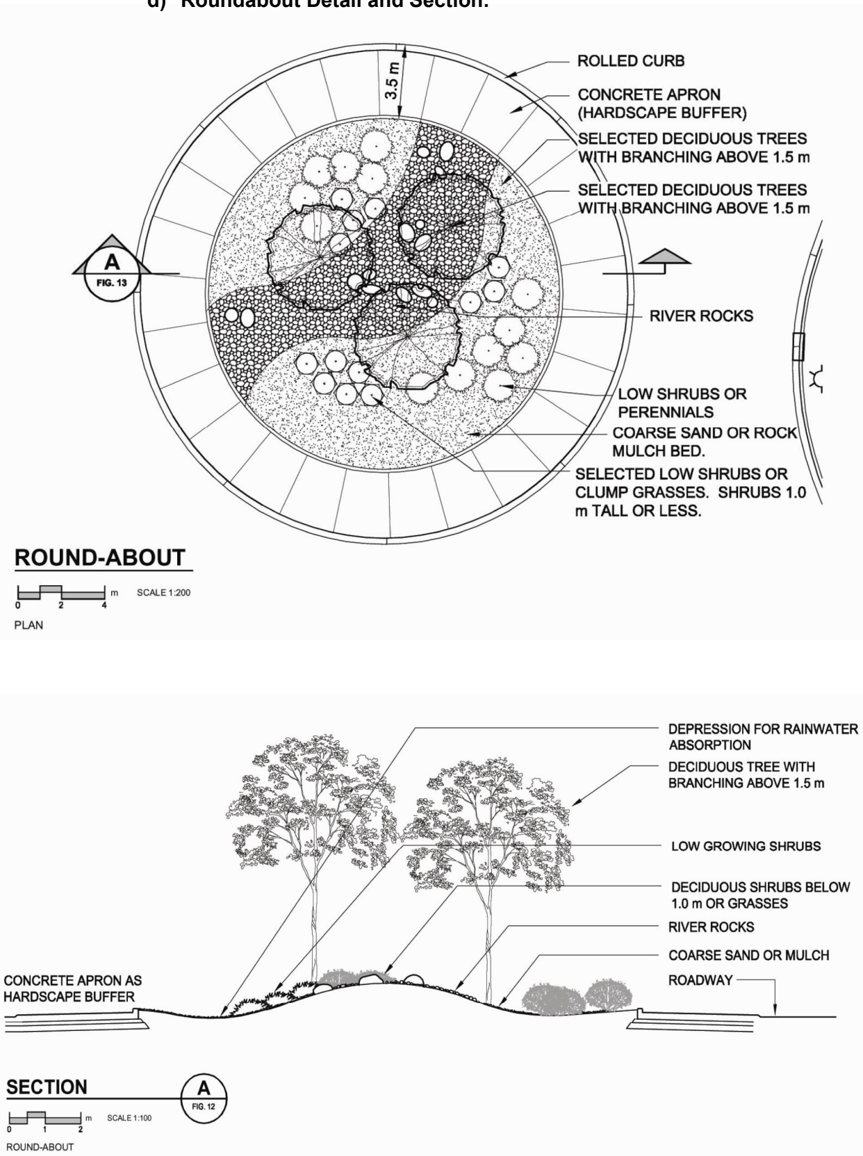
d) Roundabout Detail and Section:
